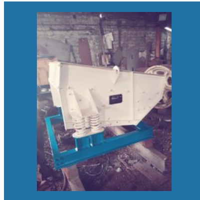
GC-VF-815 Vibrating Feeder
